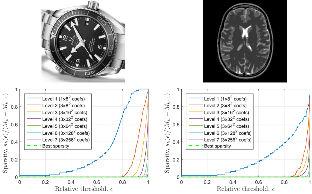
Figure 3: Relative per-level sparsities of the Daubechies-4 wavelet coefficients of two images. Here the levels correspond to wavelet scales and s_k(\epsilon) is given by (2.7). The decreasing nature of the curves for increasing k confirms (2.8).
