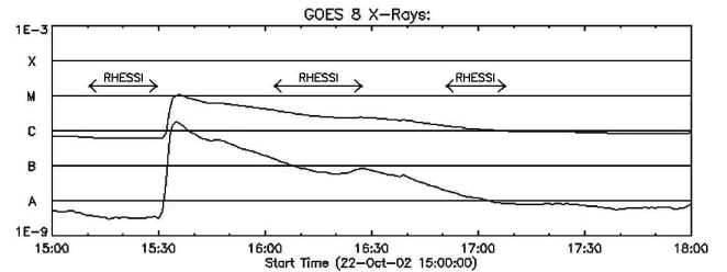
Fig. 2. Time evolution of GOES X-ray flux observed during the flare of October 22, 2002. The timings of the RHESSI observations (three orbits) are indicated. THEMIS observed continuously between 15:41–17:35 UT. TRACE and VTT/MSDP observations were performed during whole flare.
