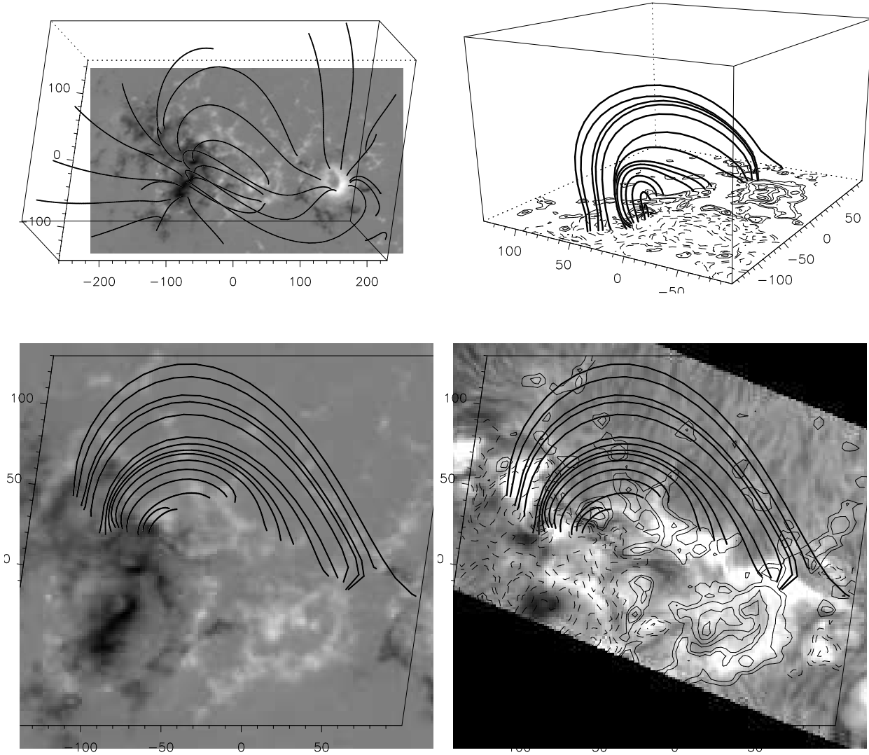
Fig. 11. ( top left: ) superposition of the THEMIS/MSDP Na D1 magnetogram of 12:32:02 UT with a sample of magnetic field lines resulting from the lfff extrapolation. ( bottom right: ) partial view of the flare as observed in H\alpha with the VTT/MSDP at 15:59:52 UT. The field lines are the ones which are rooted in the flare ribbons R1 and R2 as well as in the emerging bipole. ( bottom left: ) same as bottom right , except that the underlying image is the THEMIS magnetogram. ( top right: projection view of the field lines shown in the bottom panels. Continuous (resp. dashed) contours stand for positive (resp. negative) vertical fields. North is toward the left.
