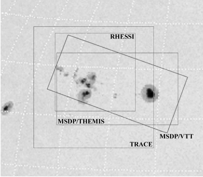
Fig. 3. Approximate orientation of FOVs of different observations used in the analysis of the flare of October 22, 2002. The north is up. For RHESSI we marked the part of FOV which was used in our analysis.
