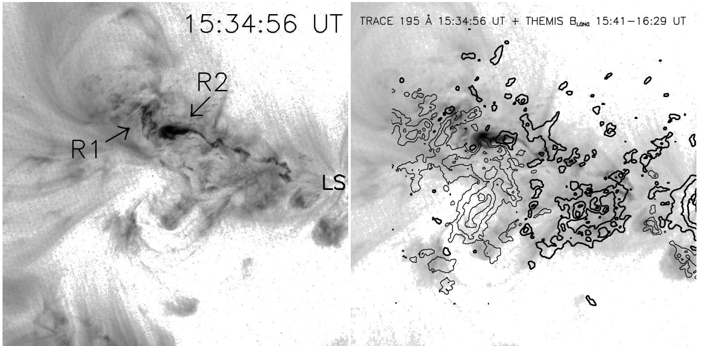
Fig. 8. TRACE 195 Å image of the AR 0162 at 15:34:56 UT. R1 and R2 denote the two main ribbons of the flare and LS marks the leading spot of the AR 0162 (left panel). In the right panel we present the contours of longitudinal magnetic field of the AR 0162 observed with THEMIS in the Na I D_1 spectral line at 15:41–16:29 UT. Thick and thin contours denote respectively the positive and negative polarity magnetic field.
