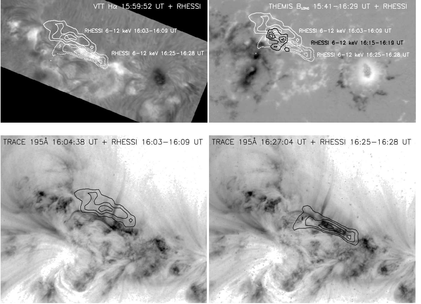
Fig. 9. VTT/MSDP image of the H \alpha flare in the AR 0162 at 15:59:52 UT (left upper panel) and the longitudinal magnetic field deduced from THEMIS/MSDP observations (15:41–16:29 UT) in the Na I D 1 spectral line at 100 mÅ from the line centre (right upper panel) overlaid with the contours of the X-ray structures observed by RHESSI at 16:03–16:09, 16:15–16:19 and 16:25–16:28 UT (right upper panel). In the lower panels we present TRACE 195 Å images of the AR 0162 (16:04:38 and 16:27:04 UT) overlaid with the contours of the X-ray structures observed by RHESSI at 16:03–16:09 and 16:25–16:28 UT time intervals.
