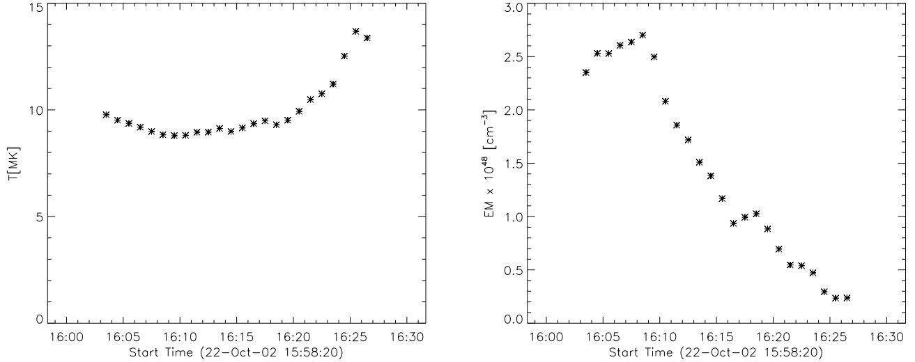
Fig. 13. The time evolution of the temperature T and emission measure EM of the flare on October 22, 2002. These parameters were obtained from fitting the observed RHESSI spectra with the model.
