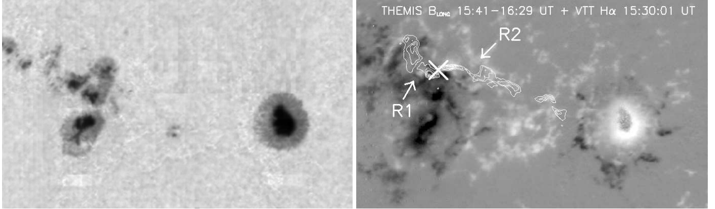
Fig. 1. Image of AR 0162 obtained from THEMIS/MSDP observations taken between 15:41 and 16:29 UT in the Na I D 1 spectral line wing at 200 mÅ from the line centre (left panel). In the right panel we present the line-of-sight (LOS) magnetic field deduced from I and V Stokes profiles at 100 mÅ from the Na I D 1 line centre overlaid with the contours of the H \alpha flare observed by VTT/MSDP at 15:30:01 UT. The field-of-view (FOV) is 400'' \times 250''. The cross denotes the place separating two main ribbons R1 and R2.
