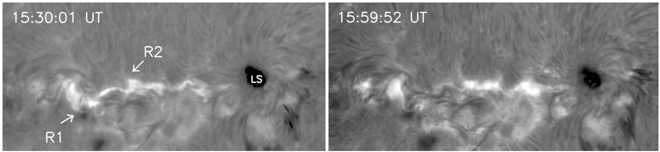
Fig. 7. The flare of October 22, 2002 observed in H\alpha line by MSDP/VTT spectrograph. The FOV is 340'' \times 200'' . R1 and R2 denote the two main ribbons of the flare. LS marks the leading spot of the AR 0162.
