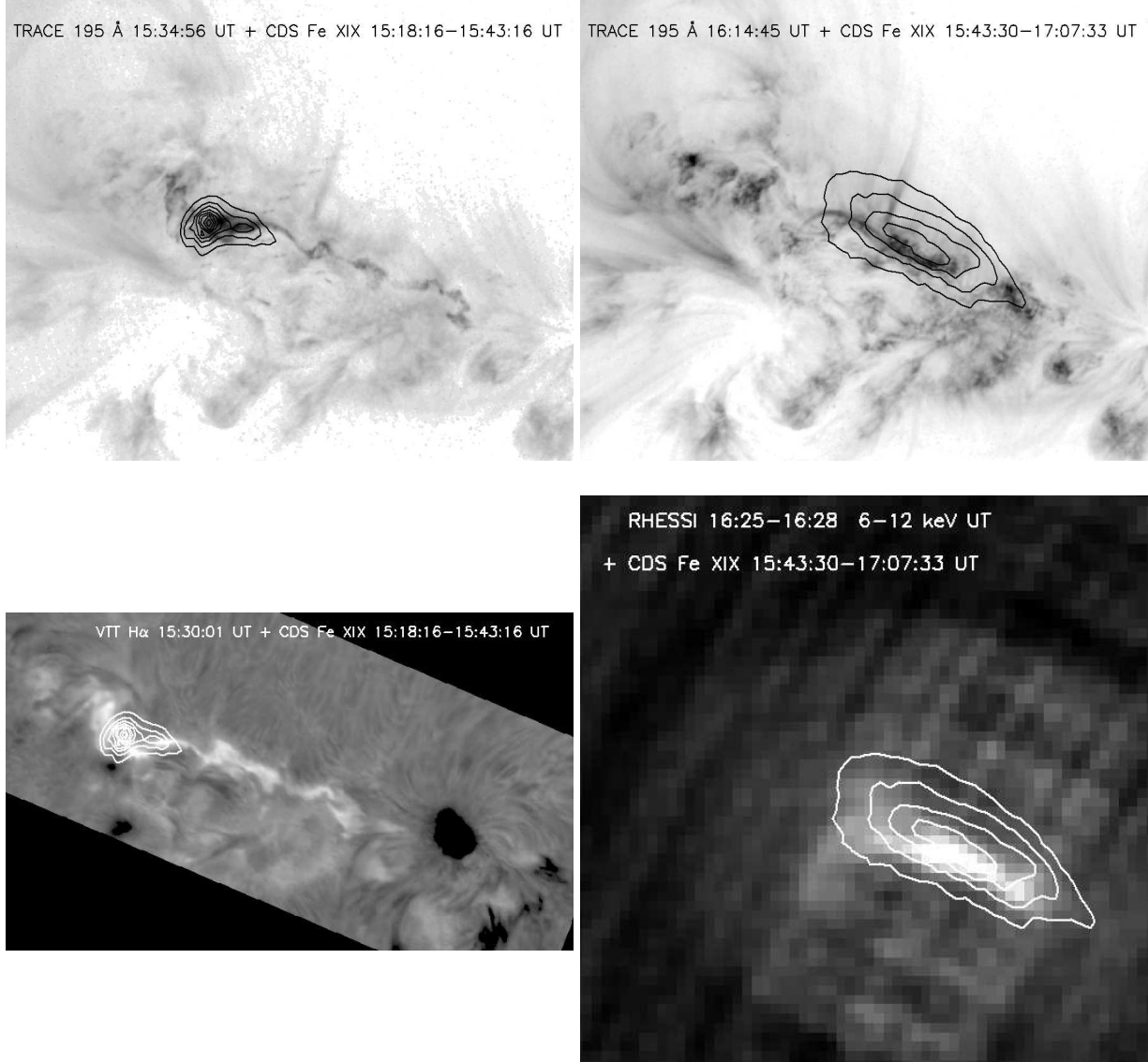
Fig. 10. TRACE 195 Å images of the AR 0162 (15:34:56 and 16:14:45 UT) overlaid with the contours of the EUV structures observed by CDS between 15:18:16–15:43:16 and 15:43:30–17:07:33 UT in the Fe XIX line (592.2 Å) (upper panels) and VTT/MSDP image of the H \alpha flare in the AR 0162 at 15:30 UT overlaid with the contours of the EUV structures observed by CDS (Fe XIX line, 592.2 Å) between 15:18:16–15:43:16 UT (left lower panel) and RHESSI image (245'' \times 245'') reconstructed for the time 16:25–16:28 UT overlaid with CDS Fe XIX structures observed between 15:43:30–17:07:33 UT (right lower panel).
