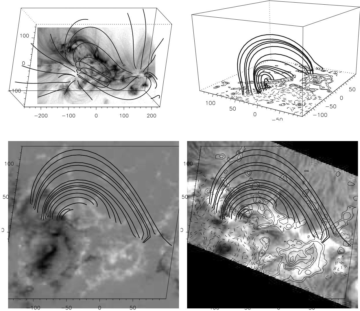
Fig. 11. ( top left: ) superposition of the TRACE 195 Å image of 16:59 UT with a sample of magnetic field lines resulting from the lfff extrapolation. ( top right: ) projection view of the field lines shown in the bottom panels. Continuous (resp. dashed) contours stand for positive (resp. negative) vertical fields. North is toward the left. ( bottom right: ) partial view of the flare as observed in H \alpha with the VTT/MSDP at 16:00 UT. The field lines are the ones which are rooted in the flare ribbons R1 and R2 as well as in the emerging bipole. ( bottom left: ) same as bottom right , except that the underlying image is the THEMIS Na D 1 magnetogram at 12:32 UT.
