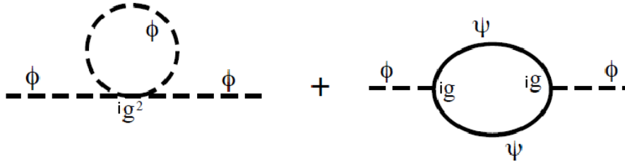
Figure 4. One loop diagrams which yield corrections to the scalar mass squared. SUSY relates the \phi^4 coupling to the Yukawa couplings \phi(\psi\bar{\psi}) and therefore ensures cancellation of the leading divergence. Note that there is another involving the trilinear diagram coming from potential terms mg\phi\phi^\dagger\phi^\dagger , but it doesn't contribute to the leading divergence.
