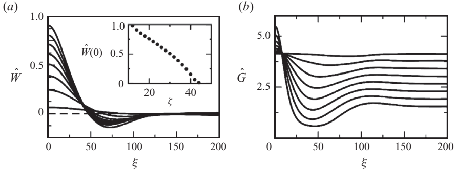
FIGURE 3. Variation of plume properties at equally spaced depths. (a) Vertical velocity \hat{w} and (b) \hat{G} , the total reduced gravity, for the parameters defined in table 1, at \zeta = 14, 18, 22, \dots, 42 . The inset of (a) shows the downward velocity at the centre of the plume as a function of depth.
