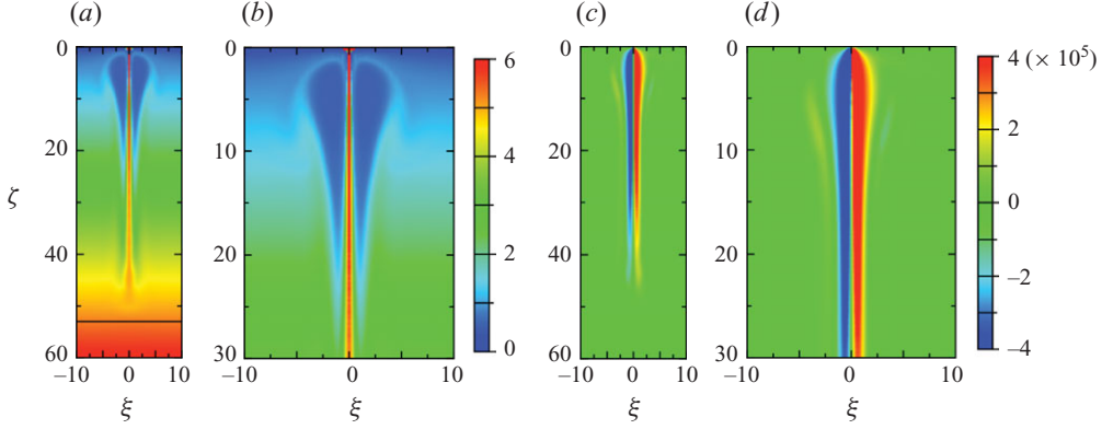
FIGURE 2. The reference base plume flow as defined in table 1. (a) Total reduced gravity \hat{G} as defined in (2.6) and (b) enlargement of source region. (c) Vorticity \hat{S} and (d) enlargement. The black line in (a) marks the penetration depth.
