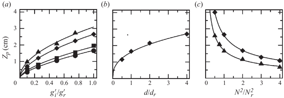
FIGURE 4. Variation of penetration depth with flow parameters, at Pe=0 , for (a) relative source reduced gravity g'_i/g'_r , (b) relative source width d/d_r and (c) relative dimensional buoyancy frequency N^2/N_r^2 , where the reference values are as defined in table 1. Numerical results are marked with the symbols, and the best-fit power laws are shown with the solid lines.
