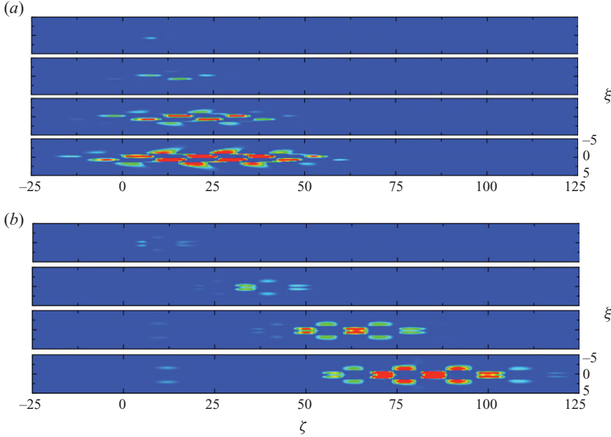
FIGURE 11. Plots of perturbation reduced gravity \tilde{g} as defined in (2.10) for a ‘reference case’ linearized flow with the parameters as given in table 1 and Re=0.05 in a parallel flow with vertical velocity and steady reduced gravity ( g_s as in (2.10)) fields extracted from a base flow plume at height \zeta_s = 16 for times \tau = 13.33, 46.67, 80 and 106.67 after the initial perturbation for (a) sinuous and (b) varicose perturbations.
