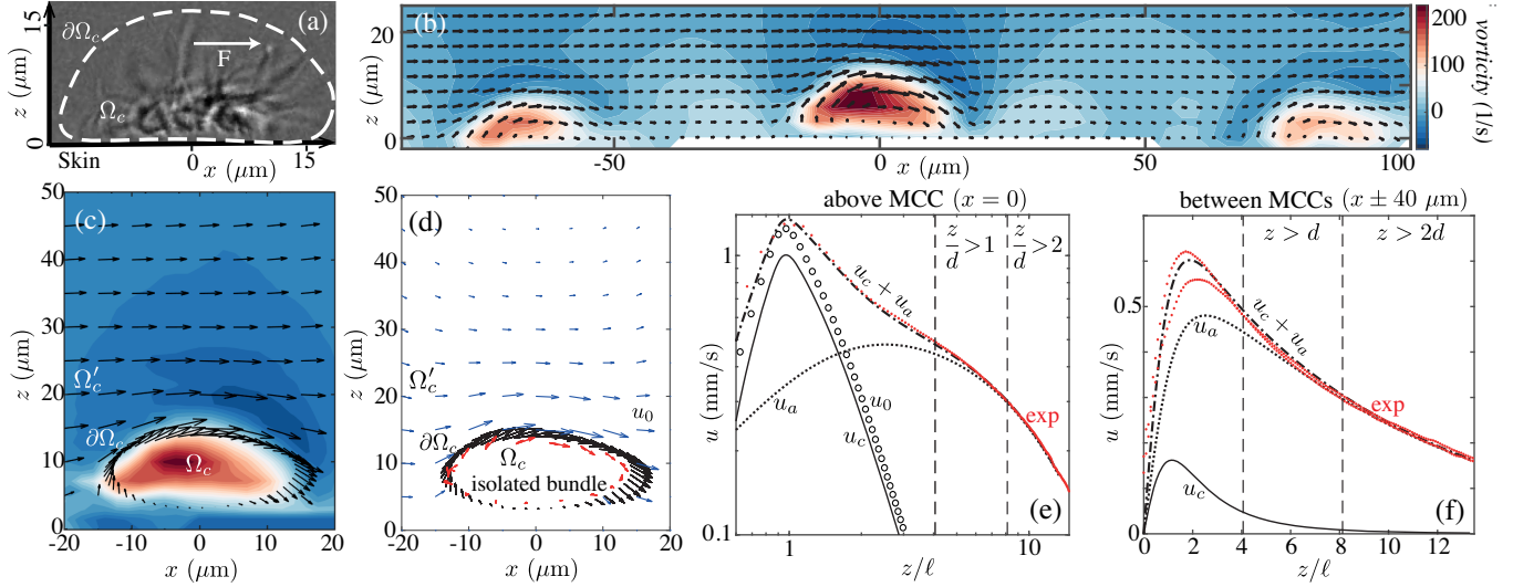
FIG. 2. Flow fields. (a) Lateral view of MCC showing (dashed) path of cilia tips and force F . (b) Experimental velocity field and vorticity in plane normal to skin near several MCCs. (c) Near an MCC, as in (b), with direction of cilia tip motion (black arrows) on \partial\Omega_c . (d) Estimated flow field u_0 for an isolated MCC (blue arrows): Point forces (red arrows) are used to fit velocity near cilia tips. Lateral velocity at (e) x, y = (0, 0) and (f) (\pm 40 \mu\text{m}, 0) in experiment (exp) and theory, with u_0 driven by an isolated bundle and u_c by a bundle exposed to endogenous flow u_a (see also Figs. S2–S4 [29]).
