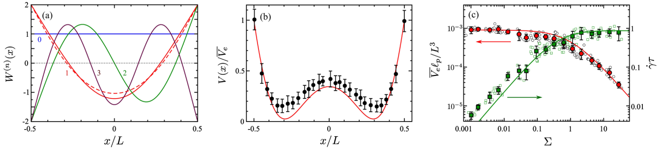
FIG. 2 (color online). Filament modes, fluctuations, and dynamics in the extensional regime \dot{\gamma} > 0 . (a) The first four orthonormal eigenfunctions W^{(n)} (solid lines) obtained from (3) for \Sigma = 0 , and W^{(1)} for \Sigma = 100 (red dashed line), illustrating the insensitivity of the fundamental bending mode shape to the tension. (b) Experimentally measured local variance as a function of position along actin filaments (symbols), and theoretical contribution from the fundamental mode (solid red line). (c) Filament-end fluctuation variance [raw data (open circles) and binned (red circles)] and scaled full relaxation time [raw data (open squares) and binned (green squares)] as a function of tension. Theoretical results are solid red and green curves, respectively.
