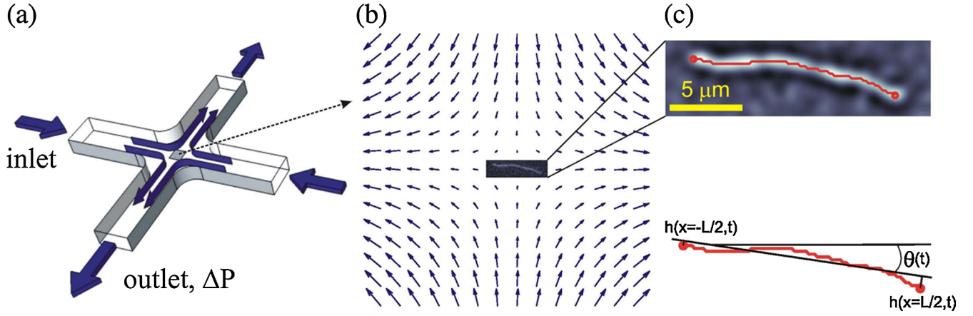
FIG. 1 (color online). Experimental setup. (a) Microfluidic cross-flow geometry controlled by a pressure difference \Delta P between inlet and outlet branches. (b) Close-up of the velocity field near the stagnation point, showing a typical actin filament. (c) Raw contour (red) of an actin filament and definition of geometric quantities used in the analysis.
