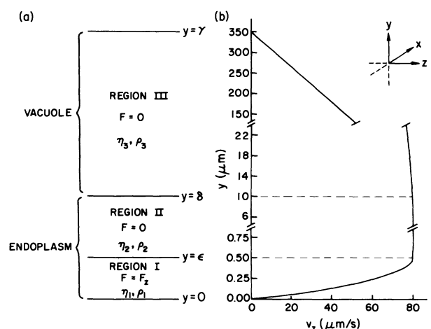
FIGURE 2 Segment of a characean internodal cell in simplified geometry for Models A and B. (a) Division of the cell into three regions, each characterized by a motive force per unit volume F , fluid viscosity \eta_i , and fluid density \rho_i . (b) Velocity profile calculated from Eqs. A-10-A-12. Parameters used in the calculation were taken from parameter set 1B of Table II. Note the scale changes along the y -axis. The x -axis points into the plane of the paper.
