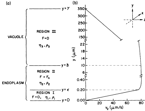
FIGURE 3 Segment of a characean internodal cell in simplified geometry for Model C. (a) Division of the cell into three regions, each characterized by a motive force per unit volume F , fluid viscosity \eta , and fluid density \rho . (b) Velocity profile calculated from Eqs. 13–16. Parameters used in the calculation were taken from parameter set 2C of Table III. Note the scale changes along the y -axis. The x -axis points into the plane of the paper.
