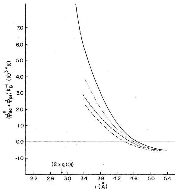
FIG. 10. Effective ion-ion potential for Rb using \epsilon_{\text{Hub}} (see Table I), q_F = 0.358(a_0^{-1}) . \Phi_{dd}^s + \Phi_{ps} ( \Phi_{BM} is very small in this region of separation). Dotted line, \bar{r}_c = 2.5a_0 , r_c(0) = 2.716a_0 , u_0 = 5 eV, \alpha_0 = 1.7\text{Å}^3 ; dashed line, \bar{r}_c = 2.5a_0 , r_c(0) = 2.716a_0 , u_0 = 15 eV, \alpha_0 = 1.7\text{Å}^3 ; dash-dotted line, \bar{r}_c = 2.716a_0 , r_c(0) = 2.716a_0 , u_0 = 30 eV, \alpha_0 = 1.7\text{Å}^3 ; solid line, \Phi_{ps} , r_c(0) = 2.716a_0 .
