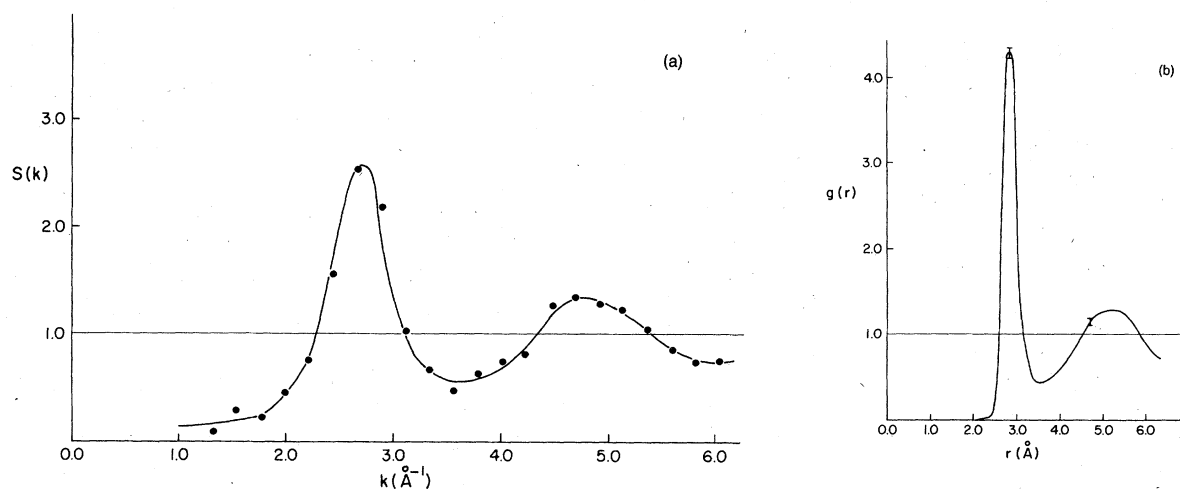
FIG. 15. (a) S(k) calculated with the potential of Fig. 2 (no core-polarization effects) using 145 particles. Here T = 296^\circ\text{K} and the density is 0.0528 \text{ (}\text{\AA}^{-3}\text{)} . (b) g(r) calculated with the potential of Fig. 2 ( T = 296^\circ\text{K} ).
