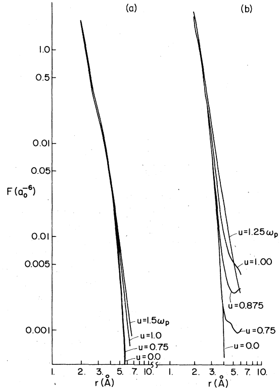
FIG. 6. (a) Form factors for Rb at q_f = 0.358 (a_0^{-1}) , \bar{r}_c(0) = 2.716 a_0 , u = (0, 0.75, 1.0, 1.5)\omega_p ( \omega_p is the electron-plasma frequency) using \epsilon_{Hub} (see Table I). (b) Form factors for Na at q_f = 0.47 (a_0^{-1}) , \bar{r}_c(0) = 1.66 a_0 , u = (0, 0.75, 0.875, 1.0, 1.25)\omega_p using \epsilon_{Hub} (see Table I).
