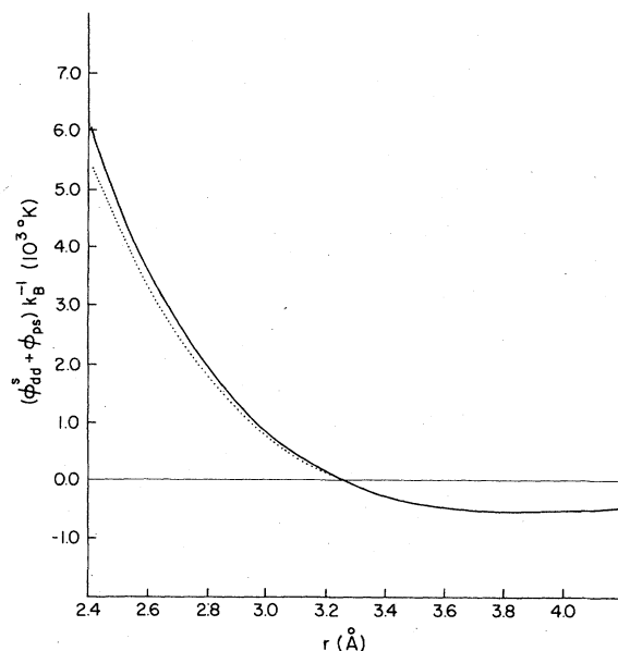
FIG. 12. Effective ion-ion potential for Na using \epsilon_{\text{Hub}} (see Table I), q_F = 0.474(a_0^{-1}) , \Phi_{dd}^s + \Phi_{ps} ( \Phi_{BM} is very small in this region of separation). Dotted line, \bar{r}_c = 1.66a_0 , r_c(0) = 1.66a_0 , u_0 = 30 eV, \alpha_0 = 0.2\text{Å}^3 ; solid line, \Phi_{ps} , r_c(0) = 1.66a_0 .
