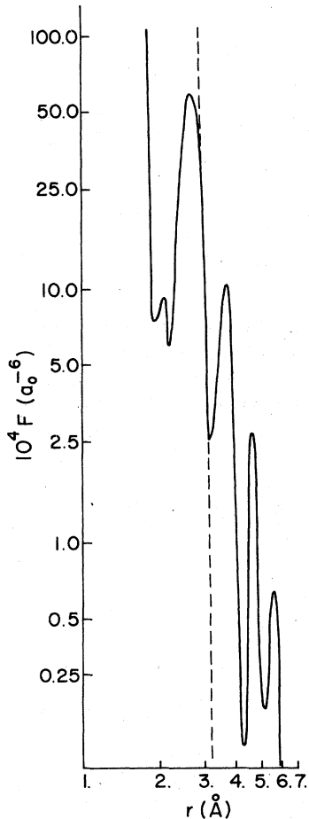
FIG. 5. Form factors F [see Eq. (34)] for Ga at q_f = 0.885 (a_0^{-1}) , u = 0 and using \epsilon_{Hub} (see Table I); Solid-line, \bar{r}_c(0) = 0 ; dashed-line, \bar{r}_c(0) = 1.25 a_0 .
