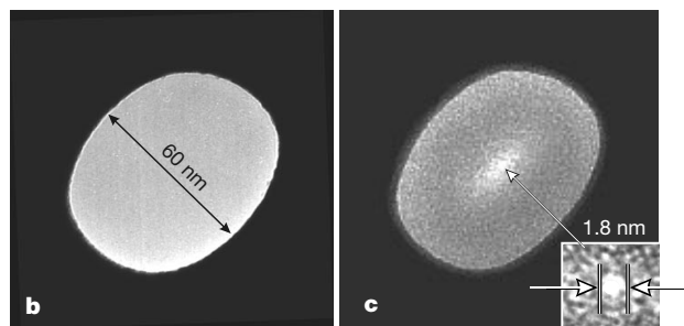
Figure 2 Sculpting a nanopore. a , Transmitted ion count rate (left axis) and pore area (right axis) versus integrated time the ion beam is on the 28 °C sample. b , TEM image of initial 61-nm diameter pore made by FIB in a 500-nm \text{Si}_3\text{N}_4 membrane. c , TEM image of the same sample after \text{Ar}^+ ion-beam exposure. Energy-dispersive analysis of X-rays in the TEM reveals the presence of Si and N in the membrane that has filled the pore, although the precise composition has not been quantified. Because the transmitted ion current is directly proportional to the area of the pore, the instantaneous pore area indicated in all figures was calculated by multiplying the initial pore area (determined by TEM) by the ratio of the instantaneous to initial transmitted ion current. Temperature, 28 °C. Flux, 28 \text{ Ar}^+ \text{ s}^{-1} \text{ nm}^{-2} . Duty cycle, 200 ms/1 s.
