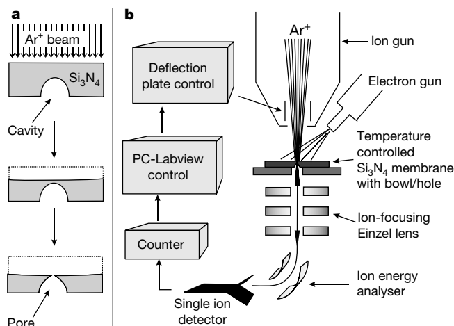
Figure 1 Strategy to make nanopores using argon ion-beam sputtering. a , Sputtering removes material from a free-standing \text{Si}_3\text{N}_4 membrane with a cavity. b , Feedback-controlled ion-beam sculpting apparatus housed in a high-vacuum chamber. a , A 500-nm-thick low-stress (~200 MPa tensile) \text{Si}_3\text{N}_4 film was deposited on a (100) silicon substrate by low-pressure chemical vapour deposition 25 . Photolithography and directional wet chemical etching of silicon were used to create a free-standing 25 \mu\text{m} \times 25 \mu\text{m} \text{Si}_3\text{N}_4 membrane 26 . Either a bowl-shaped cavity ( a ), or a single initial pore of ~0.1 \mu\text{m} diameter (not shown), was created near the centre of the membrane using, respectively, reactive ion etching 27 or a focused ion beam (FIB) machine 26 . b , A differentially pumped ion gun (VG Microtech model EX05) exposes the sample surface to an \text{Ar}^+ beam, ~0.2 mm in diameter. A Channeltron (Gallileo Optics) electron-multiplier-style single-ion detector, positioned after the sample, counts transmitted ions. Deflection plates at the exit port of the ion gun could deflect the beam off the sample or pulse the ion beam on and off the sample. A focusing Einzel lens and 60° electrostatic deflection system between sample and detector are used to suppress electron, ion and X-ray backgrounds. A 50-eV electron gun (Kimball Physics Model FRA-2x1-1) floods the sample to neutralize surface charging. A liquid-nitrogen-cooled shroud surrounds the sample and Einzel lens and a quadrupole mass spectrometer, connected to the 10^{-9} torr turbo-pumped vacuum chamber, monitors residual gas composition. A thermocouple monitors the sample holder temperature, which is adjusted with cold nitrogen gas and a resistance heater.
