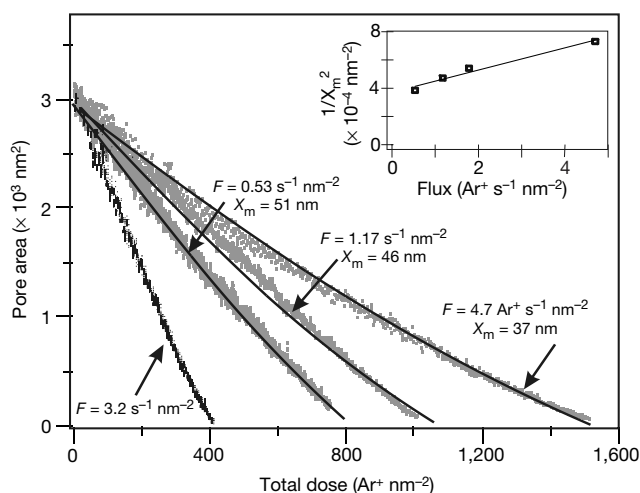
Figure 4 Flux dependence of ion-beam sculpting. Pore area versus total dose for samples exposed at different instantaneous fluxes, F , to a continuous beam (grey traces), or a pulsed beam (black traces). Duty cycle, 100 ms/1 s. The plotted black curves overlying the grey data points are predicted from the diffusion model under steady-state conditions (see text). The inset plots 1/X_m^2 versus flux, from which D is extracted. Temperature, 28 °C.
