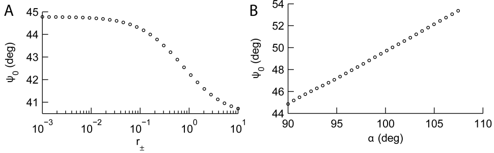
Figure 4: Dependence of the surface stagnation point angle on r_{\pm} and \alpha . (a) \alpha = \frac{\pi}{2} , r_+ = r_- , 10^{-3} \leq r_{\pm} \leq 10 , log scale in r_{\pm} . (b) r_+ = r_- = 10^{-2} , 0 < h < 0.3 .
