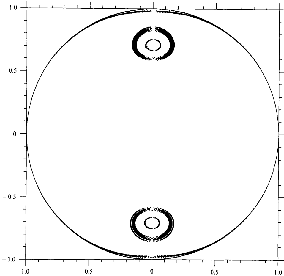
FIGURE 11. Poincaré sections (plane x = z ) of three trajectories (streamlines) of the flow (1.7) when \alpha (= \epsilon) = 0.01 and \beta = 0 . Each section consists of two parts, one close to the unit circle and the other a pair of small nearly circular bands in the interior (compare figure 10).
