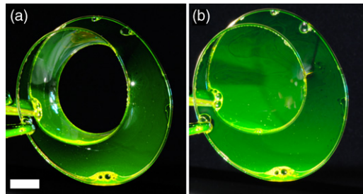
Figure 6. Topological transition of a soap film Möbius strip [24]. As its frame is gradually distorted, a critical point is reached at which the one-sided film (a) transforms rapidly to a two-sided solution (b). Scale bar in (a) is 2 cm.
