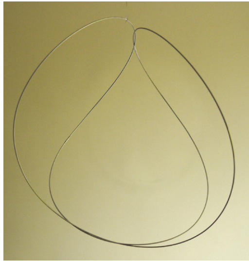
Figure 1. Minimum-energy configuration of a stiff wire in the form of a figure-of-eight knot; the two points of double contact are evident.
