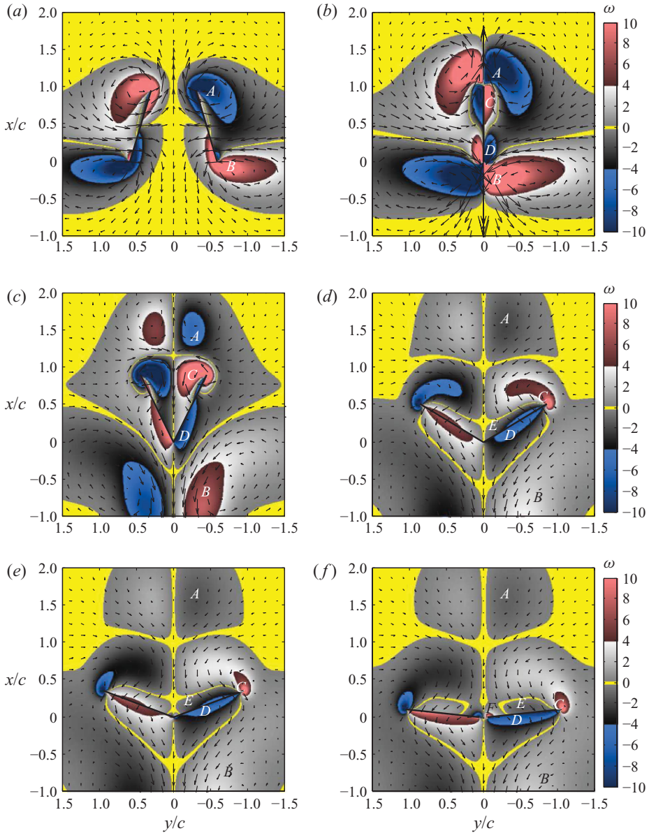
FIGURE 22. (Colour online) Vorticity (colour plots) and velocity (vector plots) during clap–fling–sweep at Re=20 . Time instants are (a) t=-0.3 , (b) t=0 , (c) t=0.5 , (d) t=1.08 , (e) t=1.25 and (f) t=1.5 . Letters A to F denote pairs of vortices generated by the two wings.
