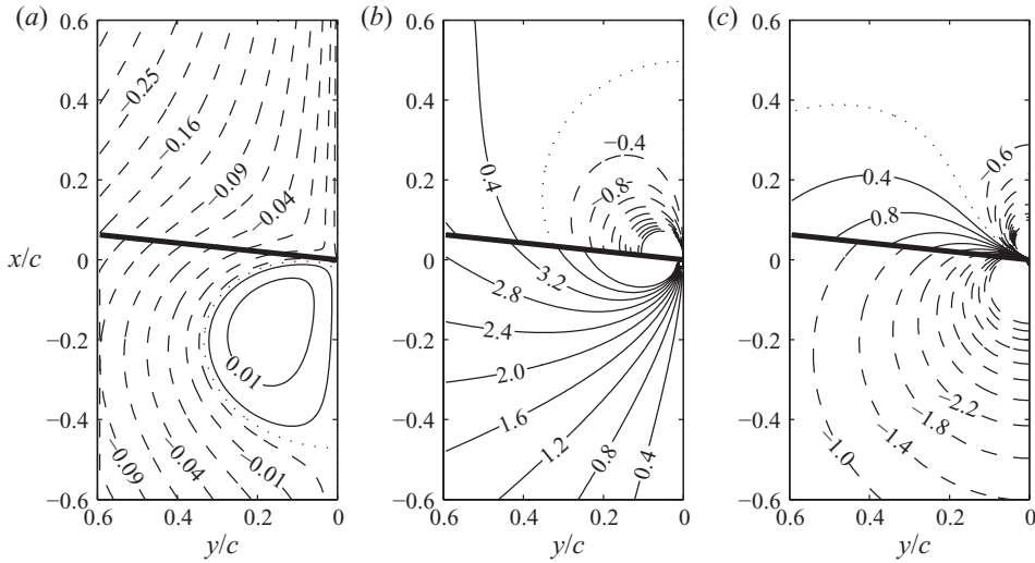
FIGURE 12. Flow during sweep as given by the local similarity solution (3.9) at t = 1.5 . (a) Streamlines corresponding to \psi \in \pm(0, 0.05^2, 0.1^2, \dots) ; (b) isolines of the vorticity drawn with a constant step \delta\omega = 0.4 ; (c) isobars drawn with a constant step \delta p = 0.4 . Contours of positive and negative values are identified using, respectively, solid and dashed lines. Dots indicate the zero isoline.
