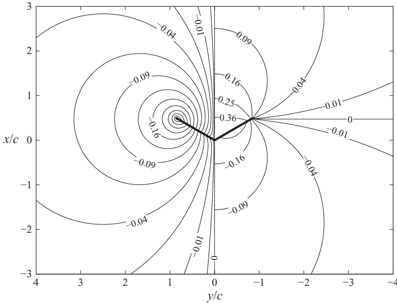
FIGURE 5. Streamlines (left half of the figure) and iso-potential lines (right half) of Lighthill's solution. The values are normalized by \Omega c^2 . The axis of symmetry is the x -axis, for consistency with (2.9).
