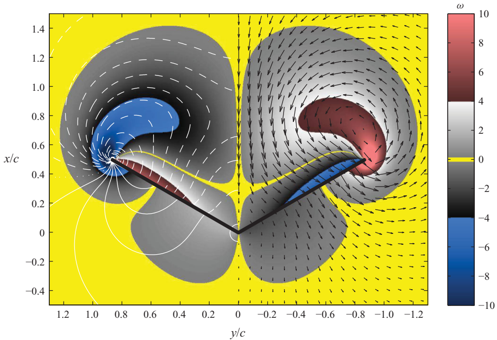
FIGURE 21. (Colour online) Flow during fling at Re = 20 , visualized at t = 1.08 . Colour plot displays the vorticity. Vector plot on the right half of the figure shows the velocity. Contours on the left half are isobars drawn with a constant step \delta p = 0.125 . Their positive, zero and negative values are identified with, respectively, solid, dotted and dashed lines.
