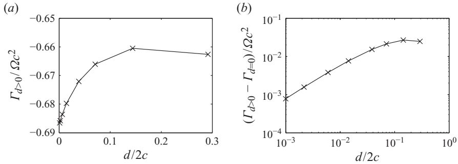
FIGURE 7. (a) Circulation \Gamma_{d>0} around the wing (normalized by \Omega c^2 ); (b) its difference with respect to \Gamma_{d=0} obtained from Lighthill’s model.
