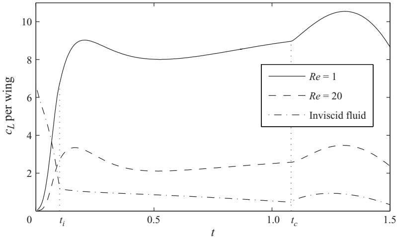
FIGURE 20. Lift coefficient per wing obtained in numerical simulations of viscous fluid flows at Re=1 (solid line) and Re=20 (dashed line). Lift coefficient in an inviscid fluid is also shown for comparison (dash-dotted).
