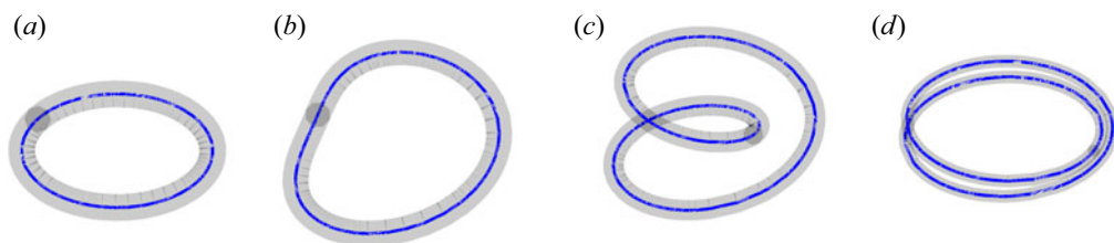
Figure 13. The stretch–twist–fold process, illustrated by the parametric equation (6.14); here stretching, twisting and folding occur simultaneously as t increases from 0 to 1. A shaded tube encloses the central curve; the cross-section of this tube decreases so that the volume of the tube remains constant. An inflexion point occurs at s = 0 at time t = 0.2 . (a) t = 0 . (b) t = 0.2 . (c) t = 0.75 . (d) t = 0.95 .
