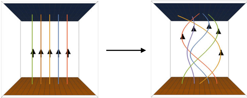
Figure 20. Model for the formation of current sheets: movement of the end points of an initially uniform field produces braids of arbitrary complexity (after Parker 1994).
