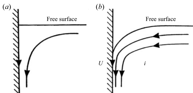
Figure 8. (a) Hypothetical (but unrealistic) flow near the contact line when a flat plate is drawn into a viscous fluid with velocity U ; (b) the ‘half-cusp’ between the free surface and the plate that must occur near the contact line due to the downward drag on the fluid.
