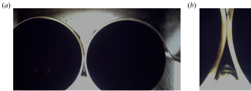
Figure 7. As in figure 6, but here the cylinders are close to each other, and only partially submerged; (a) the viscous fluid is drawn up in a layer on each cylinder and the layers interact as the fluid passes down through the gap, forming a cusp; the free surface can be seen on the right of the photo; (b) blow-up of the cusp region showing how air is drawn through the cusp in a very thin sheet forming a ‘tricuspidal’ bubble from which smaller bubbles of air are ejected into the fluid. (Photographs taken by author in 1992, but not previously published.)
