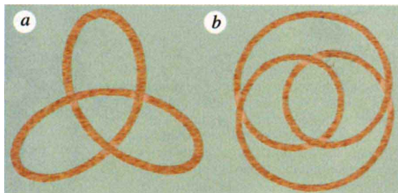
The trefoil knot, in different configurations T_{2,3} (a) and T_{3,2} (b). The trefoil is a special case of the torus knot T_{n,m} which winds n times round a torus the long way, and m times the short way.
