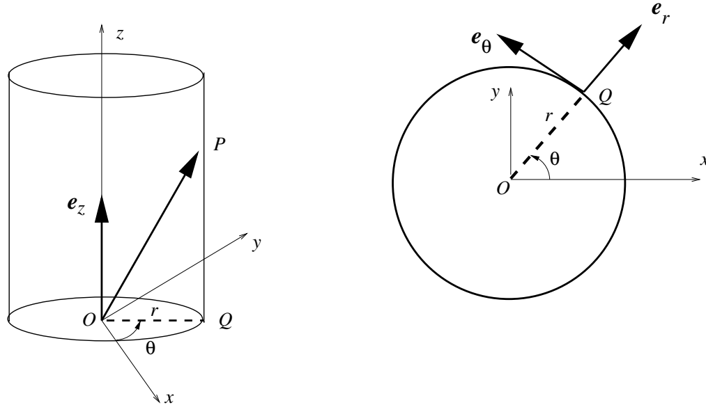
Figure 25: Diagrams illustrating the cylindrical polar coordinate system.
