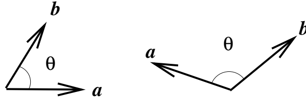
Figure 16: In the example on the left \mathbf{a} \wedge \mathbf{b} points out of the page, while in the example on the right \mathbf{a} \wedge \mathbf{b} points into the page.
