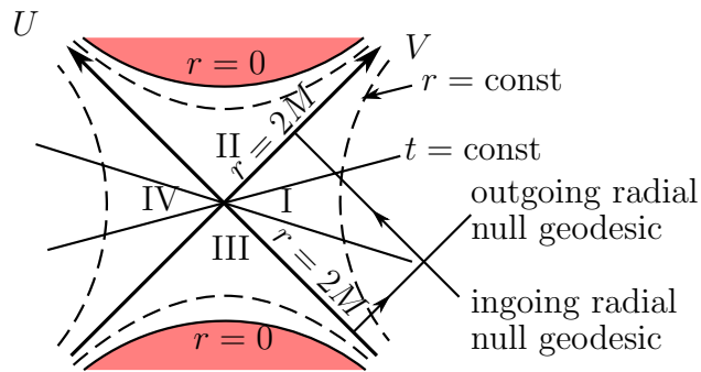
Figure 2.6: Kruskal diagram
