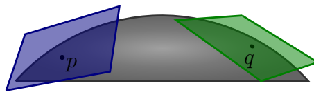
Figure 2.7: Tangent planes.
