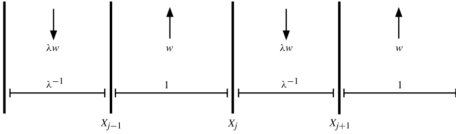
FIGURE 12. A schematic showing the interleaving flow of two distinct fluids of different densities, in columns with width ratio \lambda .
