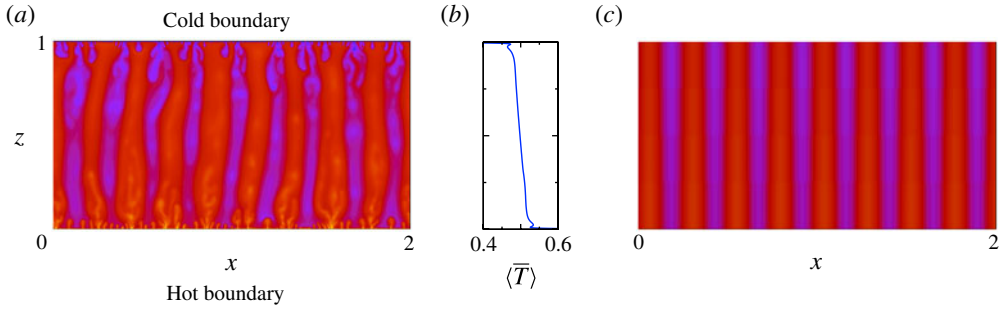
FIGURE 1. (Colour online) (a) A snapshot of the temperature field in a Rayleigh–Darcy (porous Rayleigh–Bénard) cell at Ra = 2 \times 10^4 (taken from Hewitt et al. 2012), which is dominated by vertical columnar exchange flow across the domain; (b) the corresponding temporally and horizontally averaged temperature \langle \bar{T} \rangle(z) , which shows the relatively weak linear temperature gradient across the interior of the domain; and (c) the temperature field of steady heat-exchanger flow with the same wavelength and background temperature gradient as (a).
