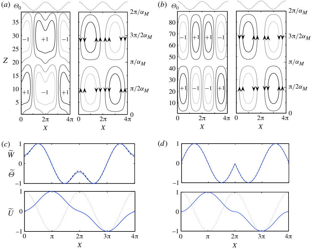
FIGURE 5. The structure of the most unstable perturbation ( a,c ) for A = 2^5 and ( b,d ) for A = 2^{20} . ( a,b ) Contours of the perturbation temperature \tilde{\Theta} (left) (scaled to unit amplitude), at intervals of 0.4, and streamlines (right) with arrows showing the direction of the flow, together with schematic profiles of the background flow \Theta_0 = W_0 (top). The perturbation is doubly periodic, with horizontal period 4\pi and vertical period 2\pi/\alpha_M . ( c,d ) Horizontal profiles of the perturbation quantities (scaled to unit amplitude): upper plots show the temperature \tilde{\Theta} (solid) and vertical velocity \tilde{W} = -\partial\tilde{\Psi}/\partial X (dashed) at Z = \pi/2\alpha_M ; lower plots show the horizontal velocity \tilde{U} = \partial\tilde{\Psi}/\partial Z (solid) at Z = \pi/\alpha_M together with the background columnar flow \Theta_0 (dotted) scaled by A . The vertical velocity and temperature perturbations are almost indistinguishable. The perturbations shown here propagate upwards; the same perturbations shifted horizontally by \pi would propagate downwards and have the same growth rate.
