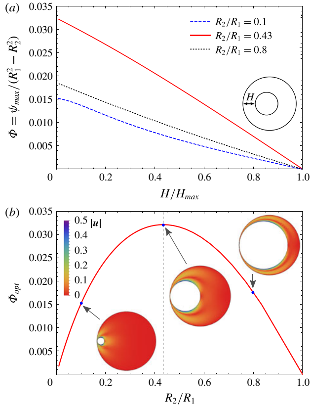
FIGURE 3. (a) Evolution of the scaled total flux in a circulation cell, \Phi = \psi_{max}/(R_1^2 - R_2^2) , with the relative gap width H/H_{max} for R_2/R_1 = 0.1 , 0.43 and 0.8 . (b) Evolution of the optimal scaled flux \Phi_{opt} (obtained for touching cylinders) with R_2/R_1 . The magnitude of the velocity field is also plotted for three cases (same as above), showing the competing effects of phoretic driving and wall hindrance on the flow.
