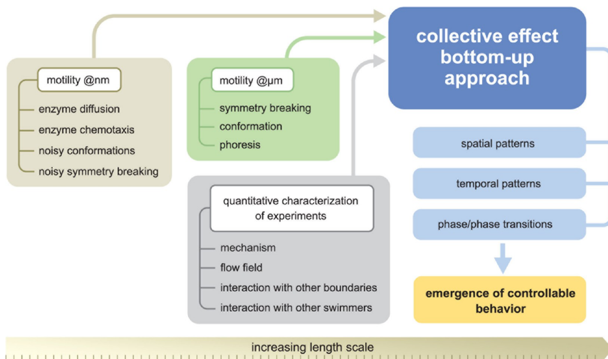
Figure 6. Multi-scale theoretical strategy to understand and control the collective behavior of micro/nanorobots. Different conceptual elements contribute to motility at nanoscale and motility at microscale. These elements, together with the quantitative characterization of various physical properties of these systems in systematic experiments, can inform a comprehensive bottom-up description of the system that enables us to make predictions of the corresponding collective properties of the system.
