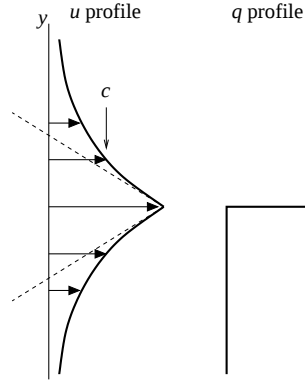
Fig. 1.8 Sketch of PV discontinuity and the corresponding velocity profile obtained by PV inversion. The step size or jet spacing L is much larger than the jet scale L_D , and we can ignore \beta and equate q_a and q . The solid velocity profile is from Eq. (1.15). The angle between the dashed lines is governed by the strength of the delta function q_j \delta(y) .
