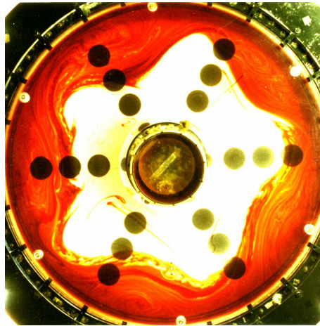
Fig. 1.1 From the laboratory study of Sommeria et al. [13]. Courtesy Dr Joël Sommeria.
