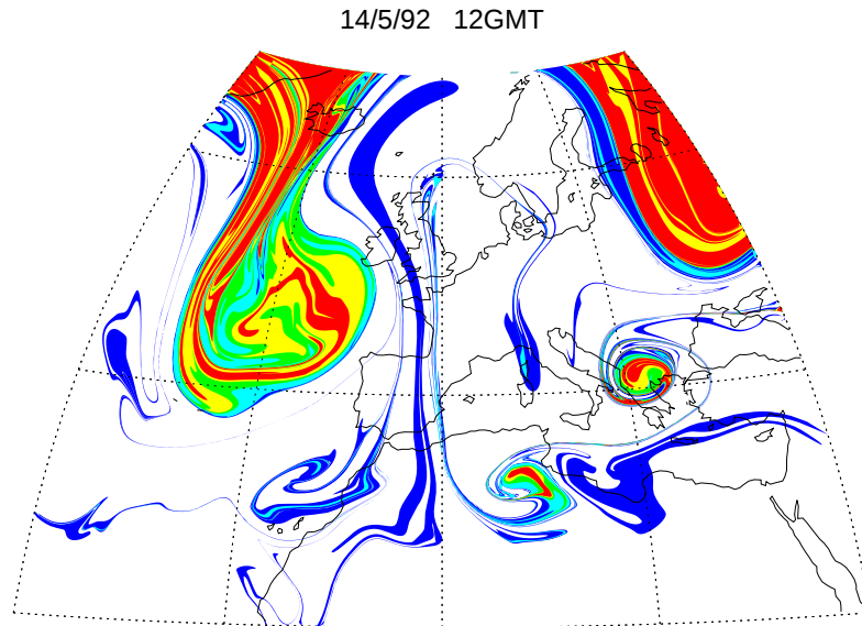
Fig. 1.4 Estimated map of Q , the exact PV defined by Eq. (1.3), on a stratification surface near 10 km altitude. From [29]. The computation assumes that material invariance of Q is a good approximation over a 4-day time interval, and uses a state-of-the-art advection algorithm and weather-forecasting data to trace the flow of high- Q stratospheric air (coloured) and low- Q tropospheric air (clear). The main boundary between stratospheric and tropospheric air marks a jet core showing large-amplitude meandering, from Greenland toward Spain and then back to northern Norway. The leakage of stratospheric air into the troposphere signals intermittent attrition of the eddy-transport barrier at the jet core. The different chemical signatures of the stratospheric and tropospheric air are easily detectable and have been demonstrated in measurement campaigns, even for fine filamentary structures like those shown [16]. The high- Q anomaly over the Balkans illustrates the “cutoff” or self-wrapping-up process that occurs when sufficiently large masses of stratospheric air overcome the barrier. The wrapping-up produces structures like that in Fig. 1.3.
