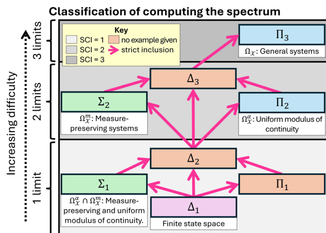
Fig. 5 | Classifications for learning Koopman spectra from trajectory data. Each SCI level indicates that solving the problem requires more complex, layered procedures. Each ‘limit’ reflects an extra data refinement. Our results establish both upper bounds (via convergent algorithms) and lower bounds (through adversarial dynamical systems) on the computational complexity of these problems. The class \Delta_{m+1} comprises problems with \text{SCI} \leq m . The \Sigma and \Pi classes characterize how verification occurs in the final limit when learning Koopman operator spectra: \Sigma corresponds to convergence from within, and \Pi to convergence from above. For finite state spaces, the problem lies in \Delta_1 , since the Koopman operator reduces to a finite-dimensional matrix whose spectrum can be computed by a single convergent algorithm with explicit rates.
