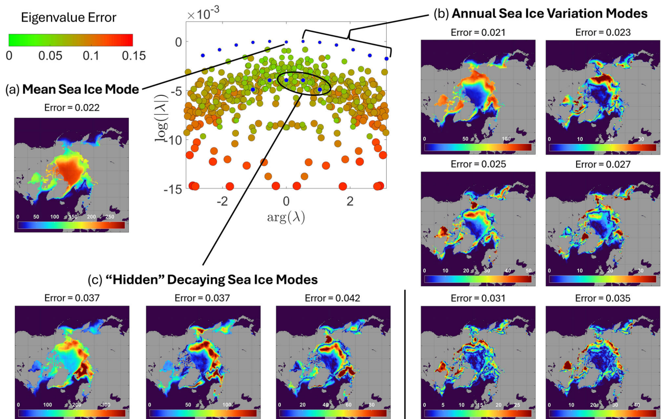
Fig. 2 | Verified eigenvalues and Koopman modes of Arctic sea ice (1979–2021) and detection of hidden modes for long-time forecasts. For each EDMD eigenvalue, our proposed method computes an associated error bound (colorbar). The displayed size of each eigenvalue is proportional to this error. While many EDMD eigenvalues are spurious, we identify 17 reliable ones (shown in blue) with small associated errors. The Koopman modes (the \mathbf{g}_j in Eq. (6), where we plot their absolute value) are categorized into three groups: a the mean sea ice concentration, corresponding to a stationary mode with eigenvalue \lambda = 1 ; b annual variation in
