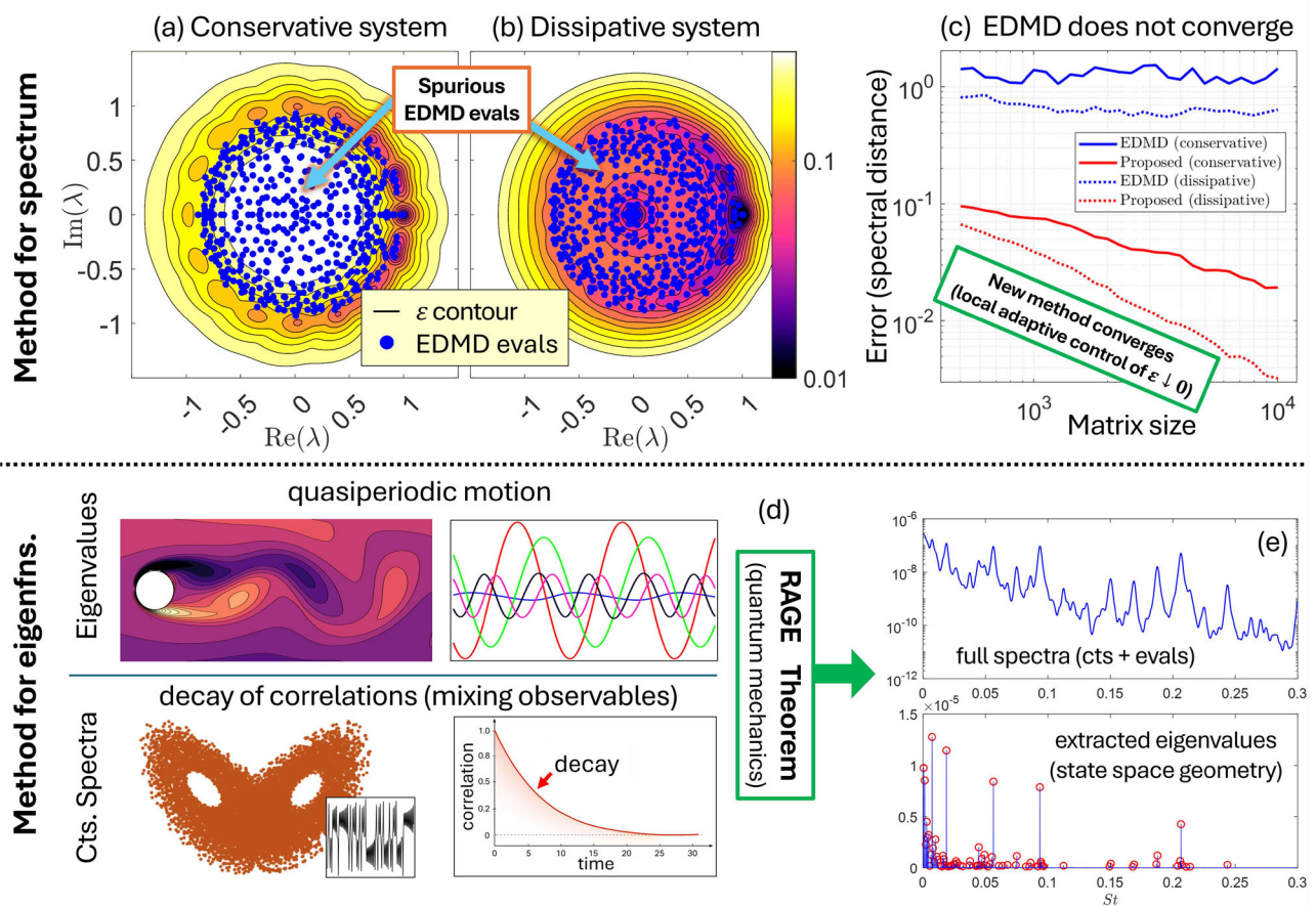
Fig. 1 | Convergent general-purpose methods for Koopman learning. Top: The method (Supplementary Algorithm 1) is benchmarked on the Duffing oscillator in conservative (a) and dissipative (b) regimes. The state-of-the-art EDMD method fails to converge (c), generating spurious eigenvalues (blue). In contrast, our approach converges reliably by adaptively computing temporally coherent observables \phi_\varepsilon and associated scalars \lambda that approximately satisfy \phi_\varepsilon(x_n) = \lambda^n \phi_\varepsilon(x_0) ( x_n is the state of the system at time n ) up to a controlled tolerance \varepsilon . The contours of \varepsilon show where approximate, near-eigenvalue behavior occurs, providing a more robust picture of dynamics. The tolerance \varepsilon is adjusted locally based on data availability and the number of observables used, yielding certified error bounds.
