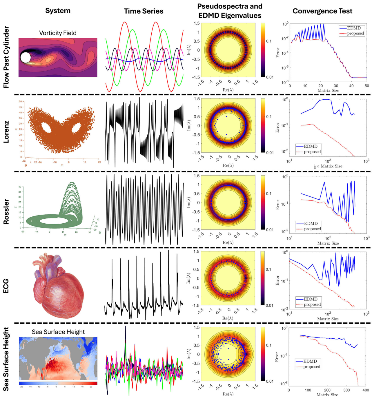
Fig. 7 | Spectral analysis of a range of analytic and real-world dynamical systems using our proposed algorithms. Each row corresponds to a different system: (i) periodic flow past a cylinder at Re = 100 , (ii) Lorenz system, (iii) Rössler system, (iv) electrocardiogram (ECG) data (Image: Heart by H. G. Wetselaar, Leiden University Libraries / Europeana, Public Domain), and (v) monthly mean sea surface height in the Northern Hemisphere (1950-present). Columns show: the system or dataset; a representative time series of observables; the computed level curves of \varepsilon for \varepsilon -approximate eigenfunctions (color scale) termed “pseudospectra” overlaid with EDMD eigenvalues (blue dots); and a convergence comparison between EDMD (blue) and our method (red, using Supplementary Algorithm 1). The
