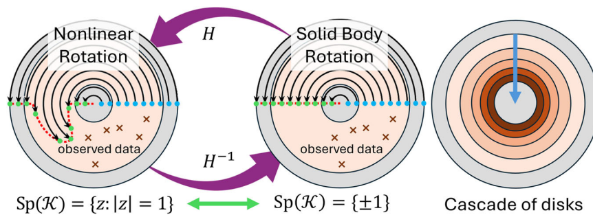
Fig. 9 | Proof idea of the impossibility result for \Omega_D . At each stage, we modify the system consistently with the observed data ("x"), ensuring it is related to a rotation, thereby drastically altering the spectrum (see green arrow). This alteration is
