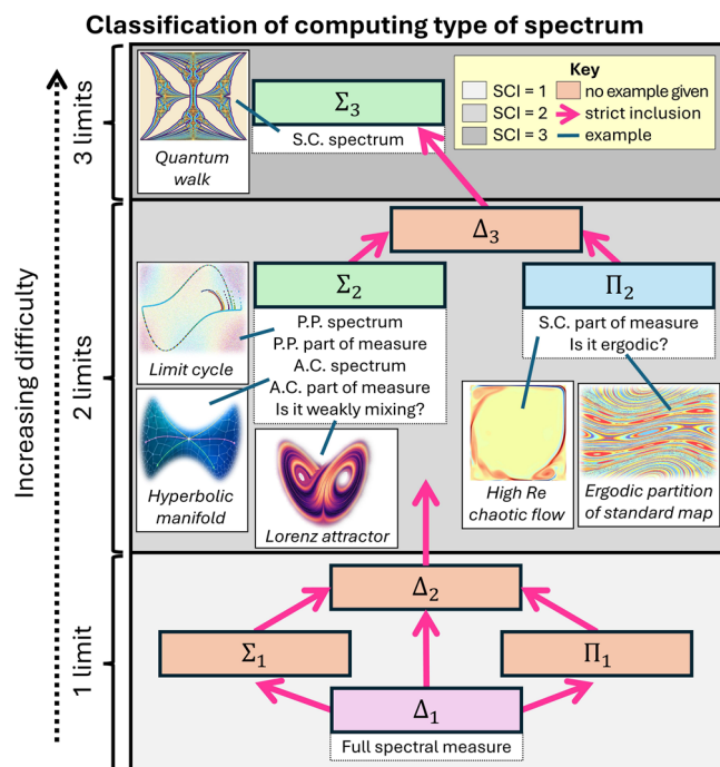
Fig. 6 | Classifications for learning spectral types (eigenvalues (p.p.), absolutely continuous (a.c.) and singular continuous (s.c.)) of Koopman operators for measure-preserving invertible systems from trajectory data. Each classification comprises an upper bound (convergent algorithms) and a lower bound (established by constructing adversarial dynamical systems). The SCI is the number of data limits needed to solve a problem. For each learning objective, we provide a representative system to emphasize that the classification fundamentally depends on the nature of the underlying dynamics. These examples illustrate how different dynamical behaviors influence the complexity of learning spectral types from data. The various classes \Delta_m , \Sigma_m , and \Pi_m are described in Fig. 5.
