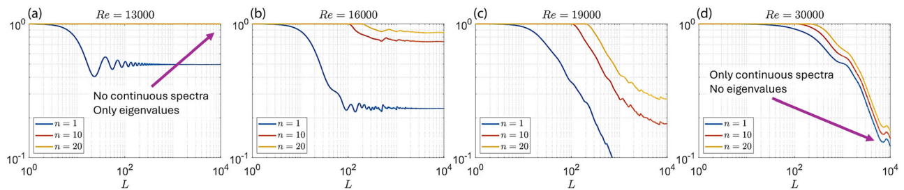
Fig. 8 | Application of Eq. (14) to the kinetic energy of a lid-driven cavity flow. The plots show \frac{1}{2L+1} \sum_{\ell=-L}^L \|\mathcal{P}_n \mathcal{K}^\ell g\|^2 (for normalized g ), which in the double limit \lim_{n \rightarrow \infty} \lim_{L \rightarrow \infty} converge to the fraction of g made up of eigenfunctions (Supplementary Algorithm 6). This double limit procedure is used to prove upper bounds.
