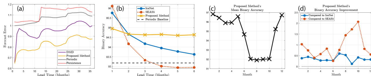
Fig. 4 | Comparison with benchmarks. a Forecast error for sea ice concentration at every grid point. Relative error of forecasted anomalies (relative to the periodic monthly climatological variance). We consider three-year forecasts initialized at each month from 2005 to 2015 and plot the average error for each lead time. The proposed method consistently outperforms DMD. b Mean binary accuracy (see text for definition) over the test years 2012–2020, shown for IceNet, SEASS, and our
