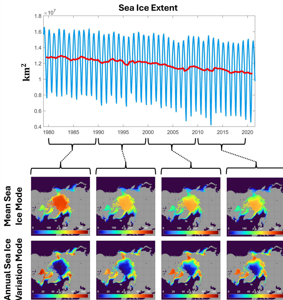
Fig. 3 | Sea ice decay and time-windowed Koopman modes. Top: Sea ice extent over the past several decades. The red curve shows the moving 12-month mean. Bottom: The absolute value of Koopman modes corresponding to the mean sea ice and annual variations over ten-year windows. The maximum error (relative
