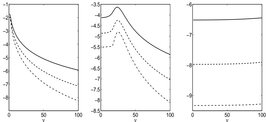
Figure 3: Relative error (in \log_{10} scale) in the computation of the Bessel function K_\nu(\nu z) , using 3 terms (solid line), 4 terms (dashed line) and 5 terms (dashed-dotted line) of the series involving Kummer U -functions. Left, \nu z = 1 + i , center \nu z = 10.1 + 20.5i and right \nu z = 100.1 + 120.5i .
