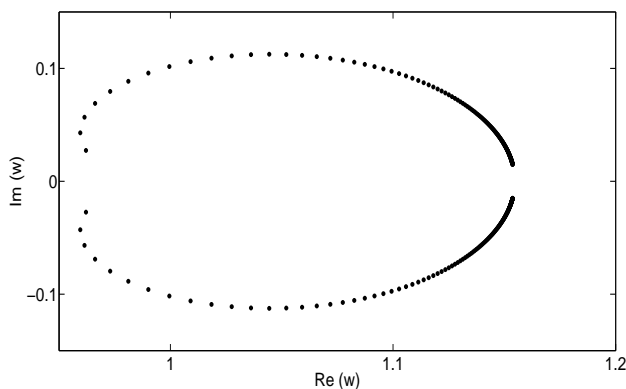
Figure 5: Saddle points s_1 (negative imaginary part) and s_{-1} (positive imaginary part), for z = 0.1, 0.2, \dots, 20 (from left to right in the graphic).
