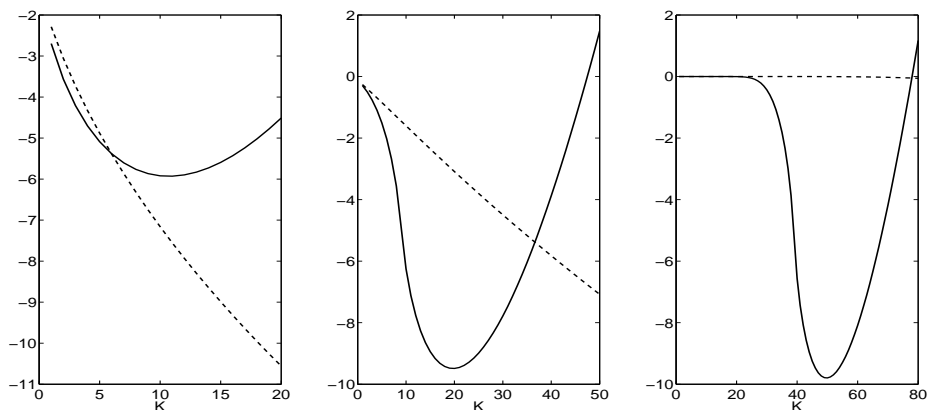
Figure 1: Relative error (in \log_{10} scale) in the computation of the incomplete Gamma, using the standard (solid line) and modified series (dashed line) with K terms and z = 10.23 . Left, a = 1.5 , center a = 10.5 and right a = 40.5 .
