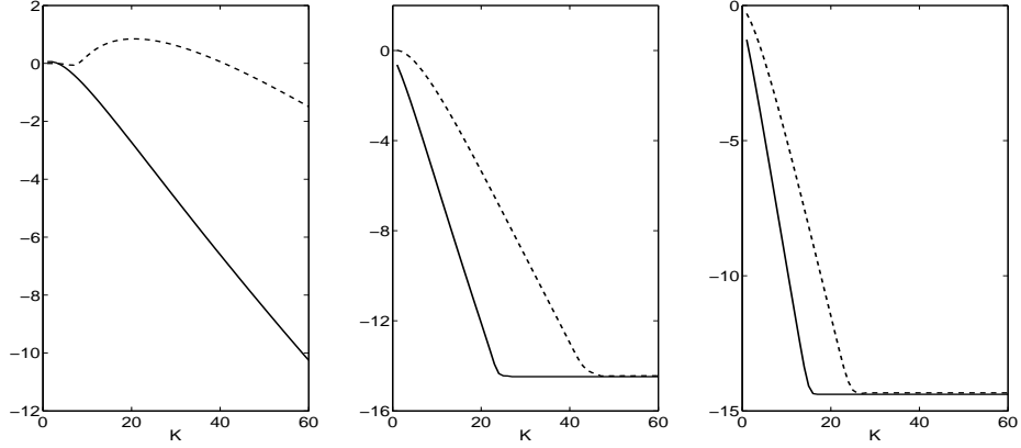
Figure 2: Relative error (in \log_{10} scale) in the computation of the Bessel function K_\nu(z) , using the series involving Kummer U functions. Left, z = 10 + 11.1i , center z = 50.1 + 42.5i and right z = 100.1 + 120.5i . Here \nu = 10.1 (solid line) and \nu = 20.1 (dashed line).
