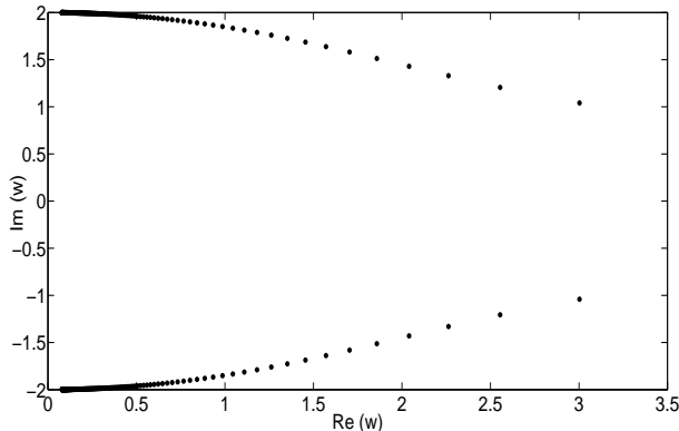
Figure 4: Saddle points w_1 (negative imaginary part) and w_{-1} (positive imaginary part), for z = 0.1, 0.2, \dots, 20 (from right to left in the graphic).
