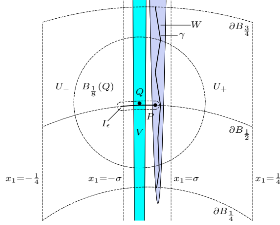
FIGURE 7. Claim 4: alternative ii^\circ
