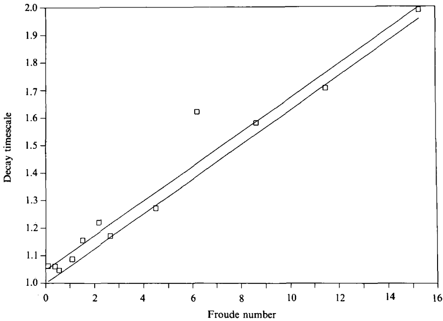
FIGURE 5. Plot of the decay constant \tau_e obtained by regression for all experiments, as a function of Froude number. The upper line indicates the best fit to the data and the lower line the theoretical behaviour.
