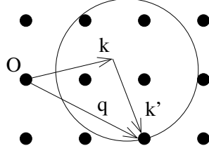
Figure 45: The Ewald sphere, drawn in the reciprocal lattice.
