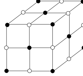
Figure 51: The reciprocal as a cubic lattice minus a basis.
