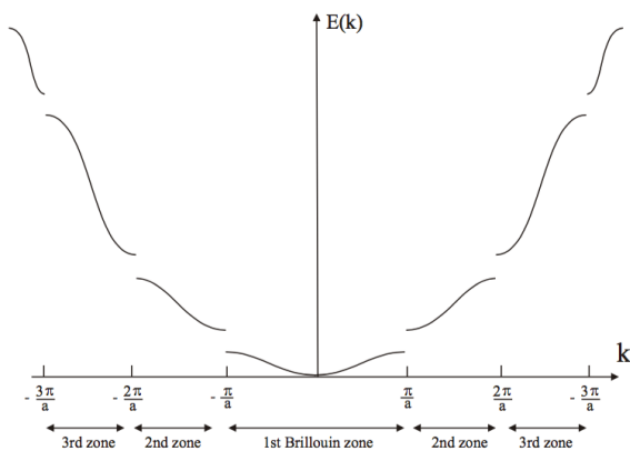
Figure 29: The extended zone scheme.
