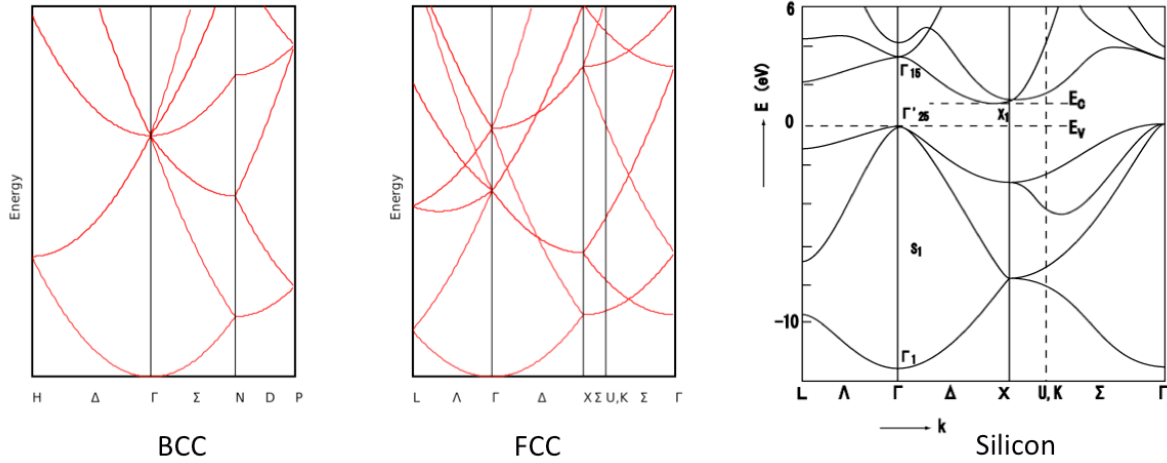
Figure 42: Free band structure (in red) for BCC and FCC, together with the band structure for silicon, exhibiting a gap.
