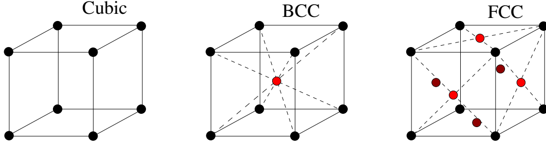
Figure 34: Three Bravais lattices. The different coloured atoms are there in an attempt to make the diagrams less confusing; they do not denote different types of atoms.
