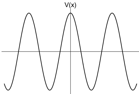
Figure 26: A periodic sine wave.
