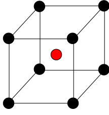
Figure 50: A BCC lattice as cubic lattice + basis.
