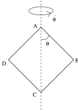
Figure 3: The rotating rhombus.
