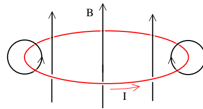
Figure 35: Lenz's law
