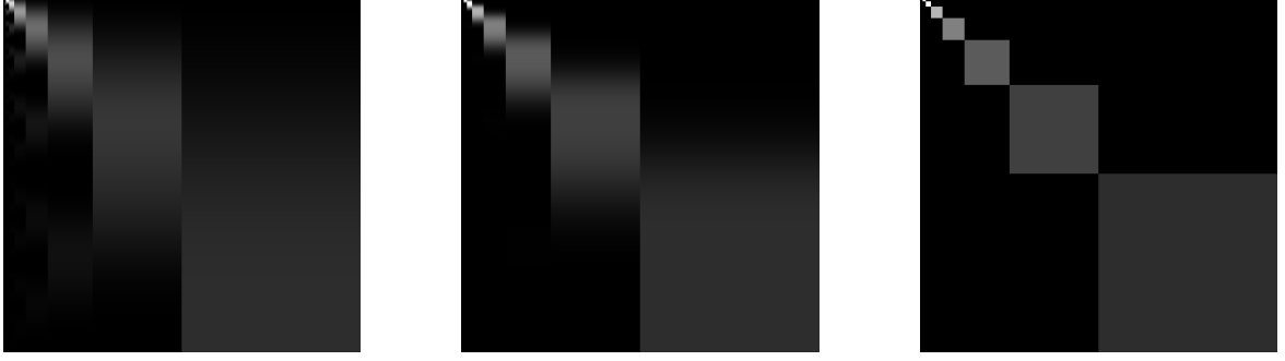
Figure 3: The three images display the absolute values of various sensing matrices. A lighter colour represents larger absolute values. (Left) \text{DFT} \cdot \text{DWT}_2^{-1} , (middle) \text{DFT} \cdot \text{DWT}_{10}^{-1} and (right) \text{HAD} \cdot \text{DWT}_{\text{Haar}}^{-1} where DFT is the Discrete Fourier Transform, HAD the Hadamard transform and \text{DWT}_N^{-1} the Inverse Wavelet Transform corresponding to Daubechies wavelets with N vanishing moments.
