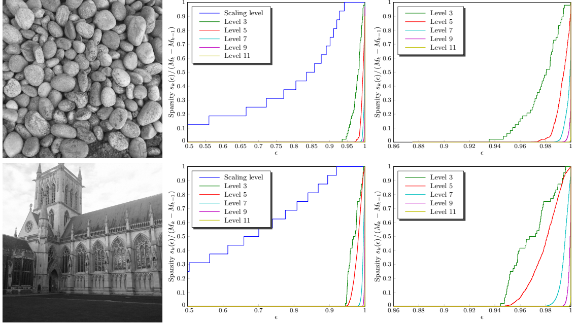
Figure 4: The relative sparsity of Haar wavelet coefficients of two image. The leftmost column displays the image in question. The middle and final columns display the values of s_k(\epsilon) for \epsilon \in [0.5, 1] and \epsilon \in [0.86, 1] respectively, where k represents a wavelet level. Of particular importance is the rapid decay of s_k(\epsilon) as k grows larger.
