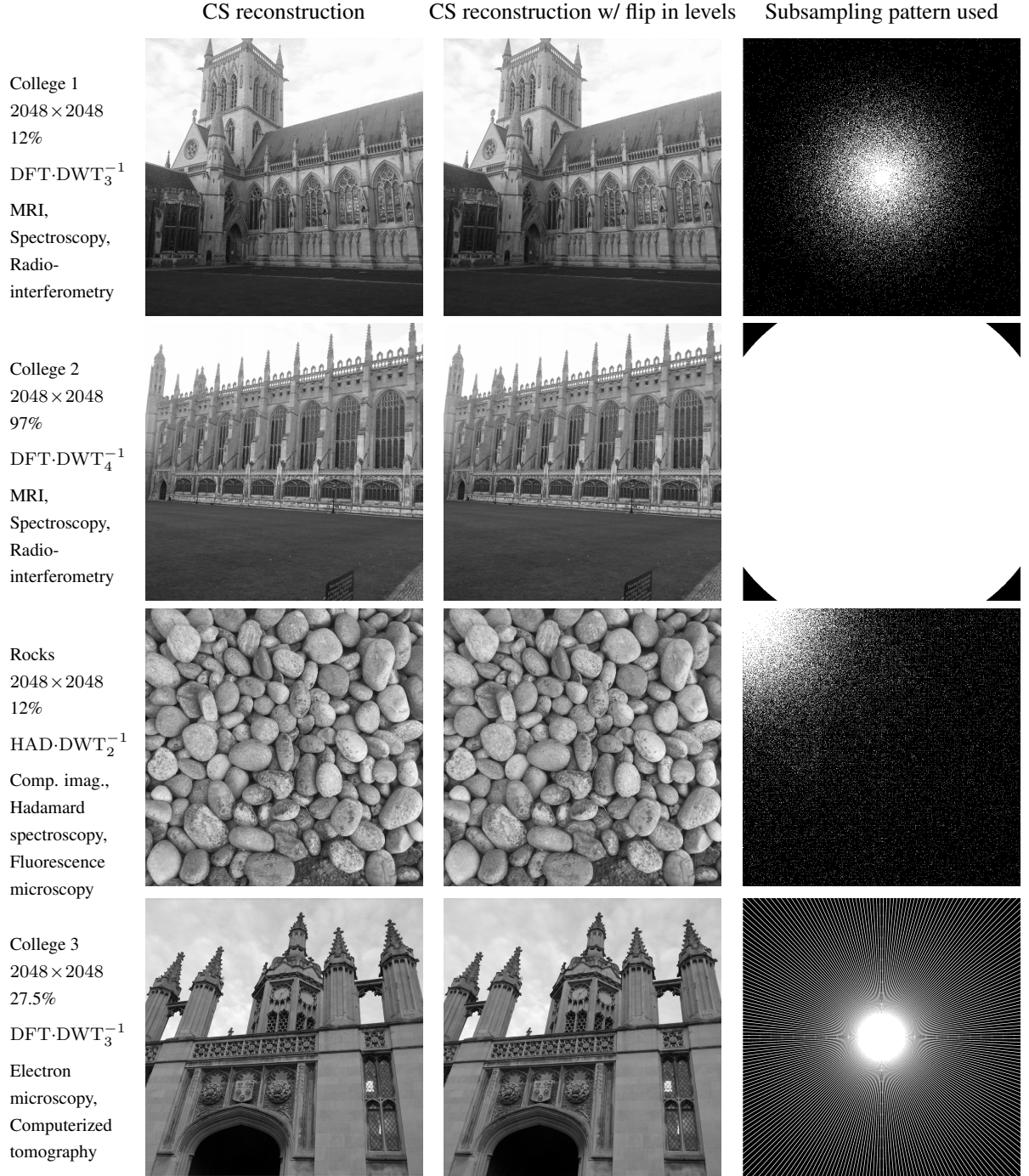
Figure 5: Standard reconstruction (left column) and the result of the flip test where the wavelet coefficients are flipped within each level (middle column). The right column shows the subsampling pattern used. The percentage shown is the fraction of Fourier or Hadamard coefficients that were sampled. \text{DWT}_N^{-1} denotes the Inverse Wavelet Transform corresponding to Daubechies wavelets with N vanishing moments.
