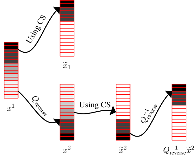
Figure 1: A graphical demonstration of the flip test for matrices which exhibit the RIP. Darker colours denote larger values.
