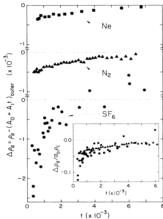
FIG. 2. Deviations of diameters from the linear fits. Inset: Deviations normalized by the critical polarizability product a_p \rho_c .
