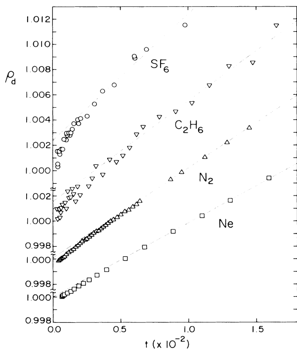
FIG. 1. Coexistence-curve diameters vs reduced temperature, with linear fits (dashed lines) determined at large t .
