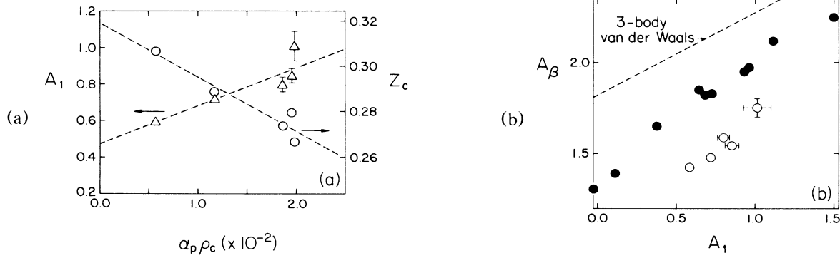
FIG. 3. (a) Diameter slope A_1 and compressibility factor Z_c vs critical polarizability product for Ne, N_2 , C_2H_6 , C_2H_4 , and SF_6 (left to right), along with linear fits (dashed lines). (b) Order-parameter amplitude A_\beta vs diameter slope A_1 for (solid dots, left to right) {}^3He , {}^4He , H_2 , Ar, O_2 , Xe, N_2O , CO_2 , NH_3 , and H_2O , from Ref. 5. Open circles (left to right) are Ne, N_2 , C_2H_6 , C_2H_4 , and SF_6 .
