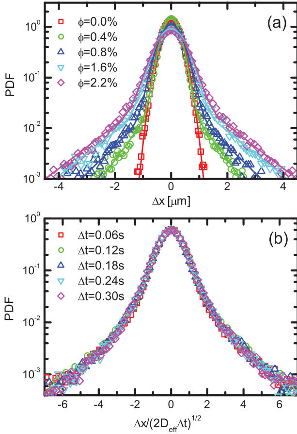
FIG. 2 (color online). Probability distribution functions for tracer displacements. (a) Overlaid PDFs at a fixed time interval \Delta t = 0.12 s, for various volume fractions, showing the broadening of the Gaussian core and appearance of exponential tails. (b) Diffusive rescaling of PDFs at \phi = 2.2\% and various time intervals, illustrating data collapse.
