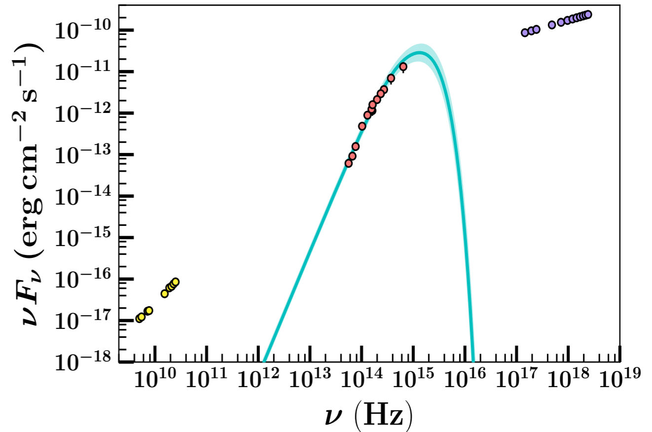
Swift J1753.5-0127: in UV
