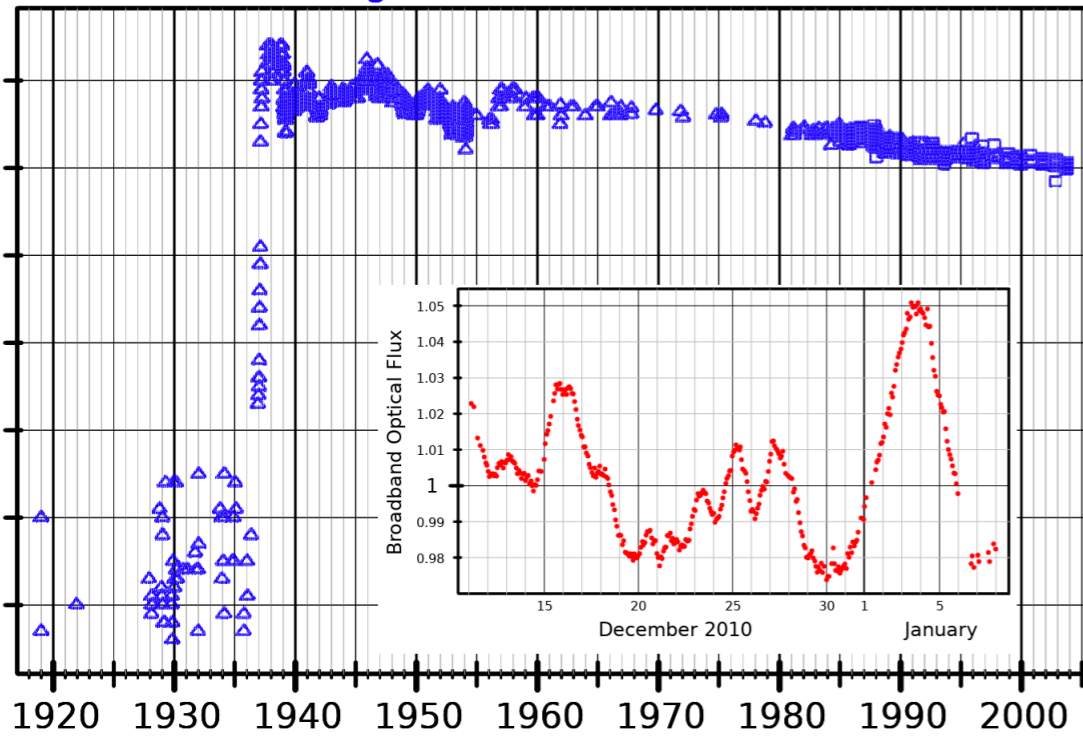
A Light Curve for FU Orionis
