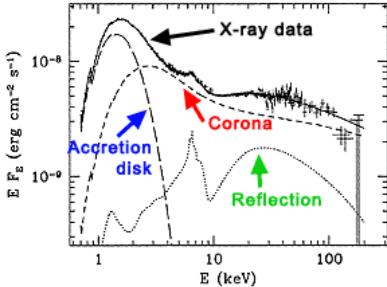
Cygnus X-2: composite spectrum in X-rays
