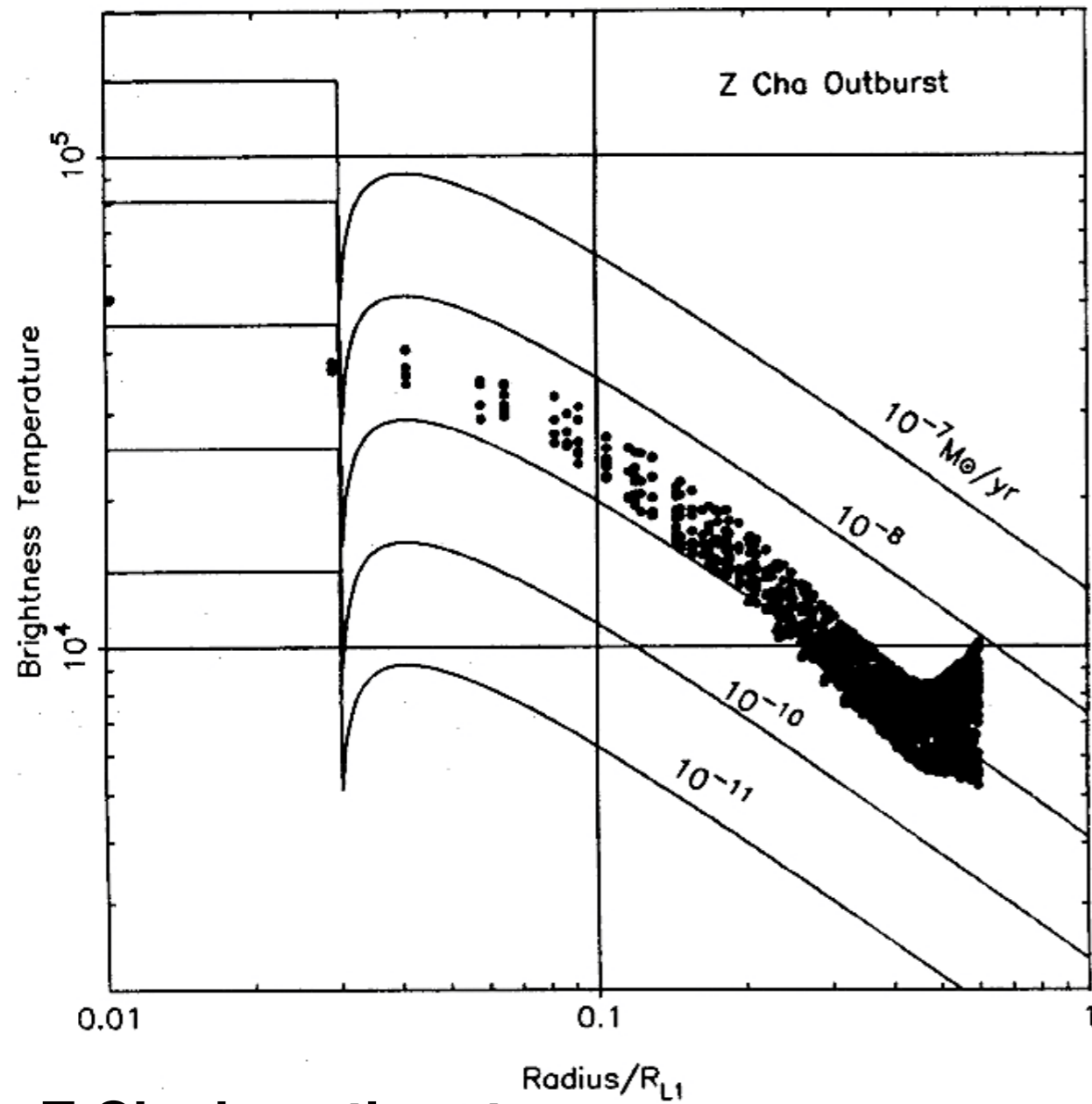
Z Cha in outburst
