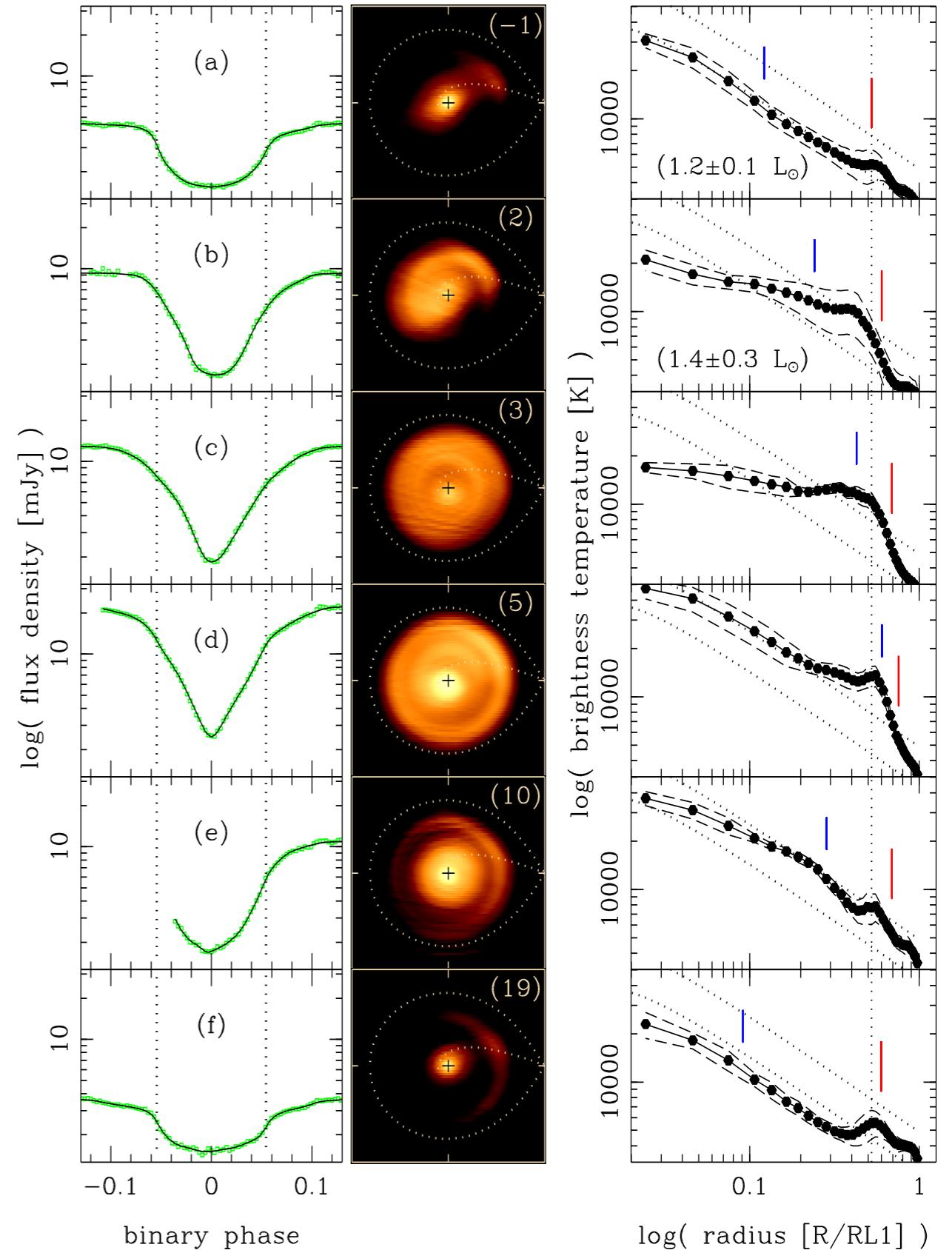
EX Dra through an outburst cycle
